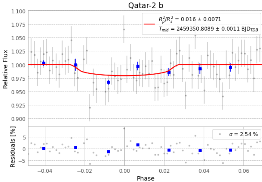
Figure 1 — FinalLightCurve_Qatar-2 b_2021-05-15.png (SHA-256 8497575e1fc280d2...)
