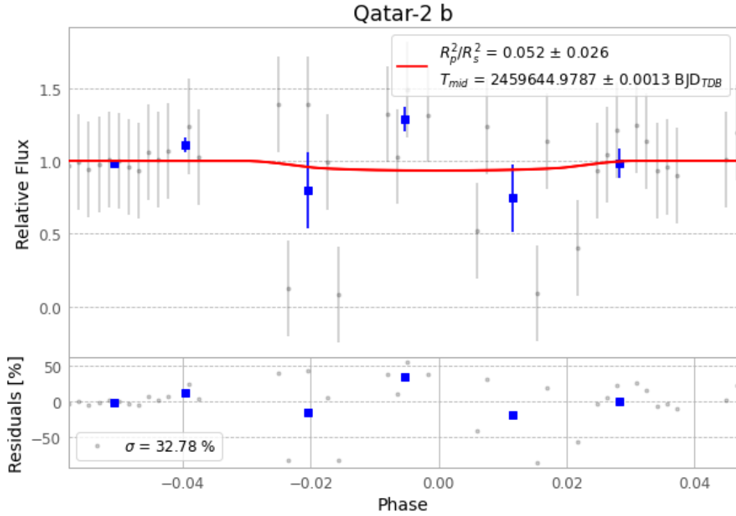
Figure 1 — FinalLightCurve_Qatar-2 b_2022-03-06.png (SHA-256 a19ad72fb8f575f3...)
