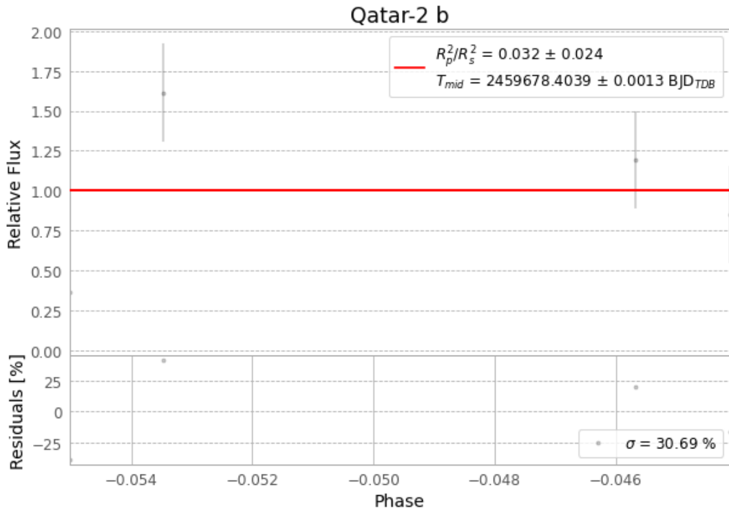
Figure 1 — FinalLightCurve_Qatar-2 b_2022-04-09.png (SHA-256 dafb9106cf2f374d...)
