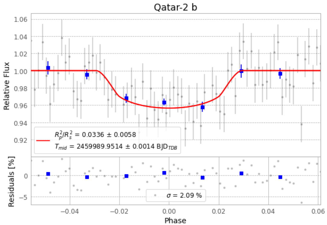
Figure 1 — FinalLightCurve_Qatar-2 b_2023-02-14.png (SHA-256 3bd965273e3308d8...)
