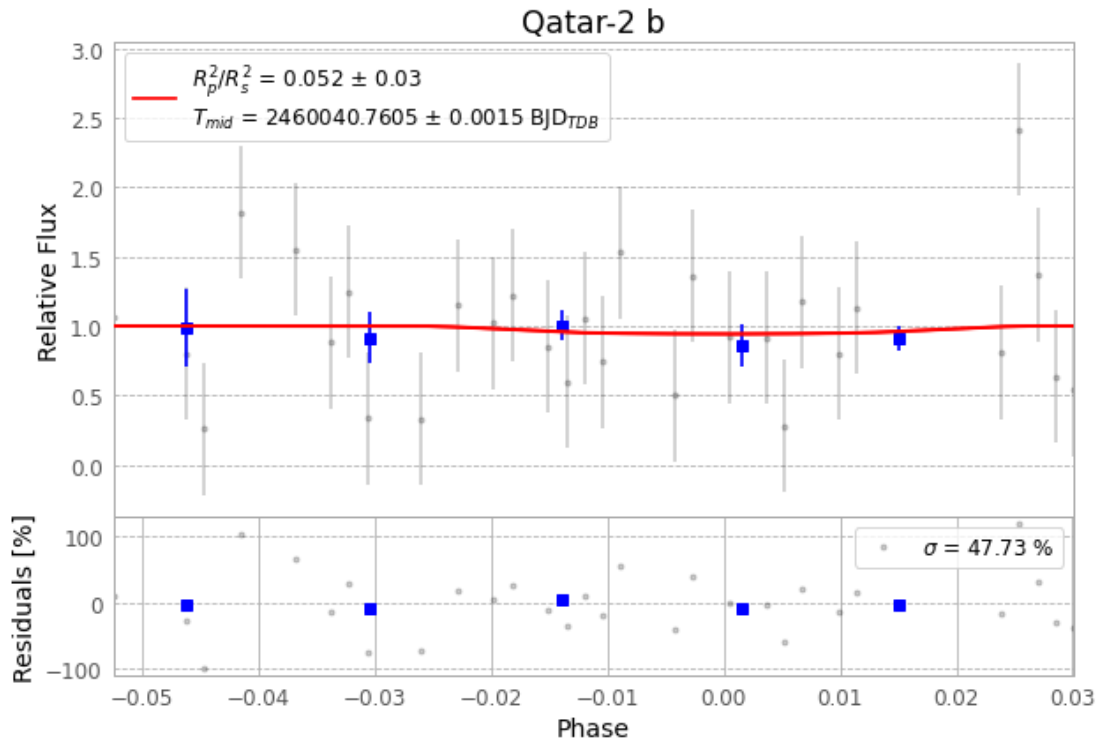
Figure 1 — FinalLightCurve_Qatar-2 b_2023-04-05.png (SHA-256 6c0fdf5c78d97adb...)
