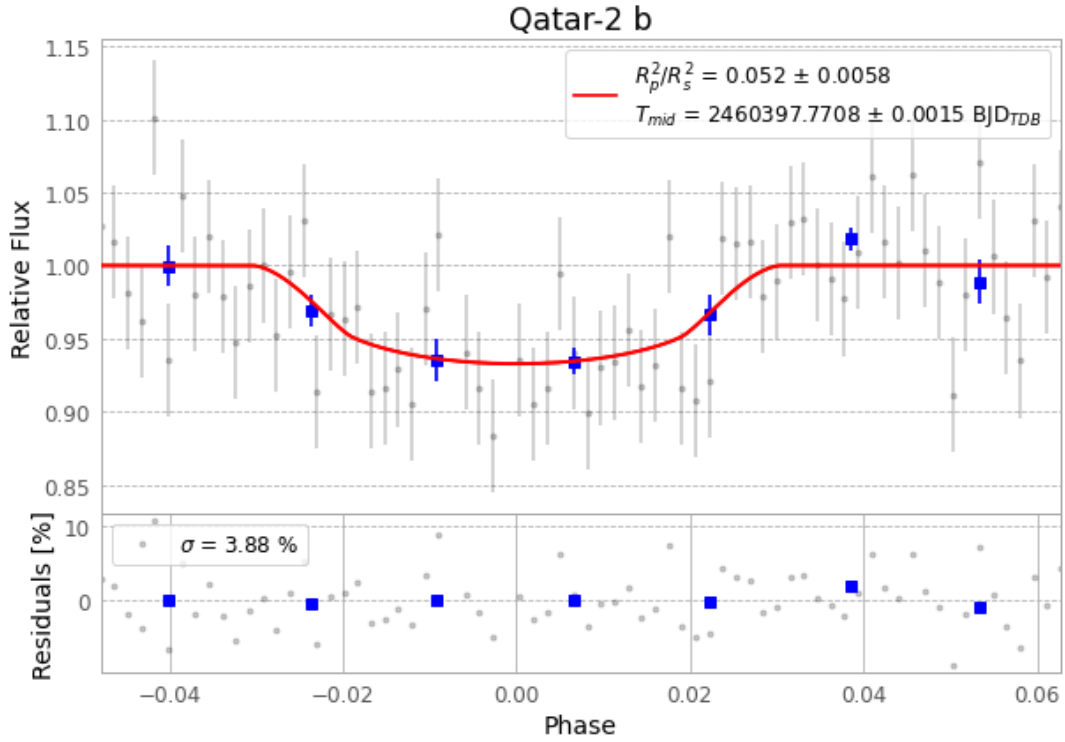
Figure 1 — FinalLightCurve_Qatar-2 b_2024-03-27.png (SHA-256 f5b56346e59d0bdc...)
