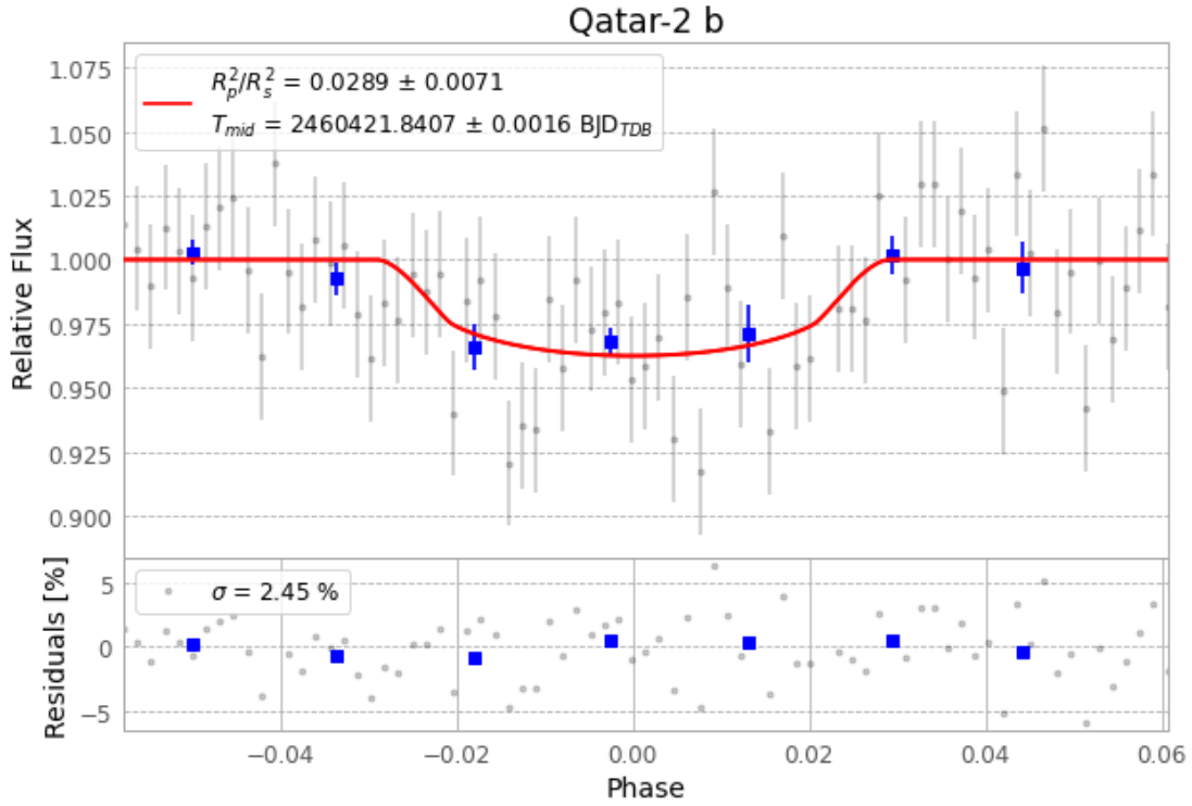
Figure 1 — FinalLightCurve_Qatar-2 b_2024-04-20.png (SHA-256 066b2d38008c6c55...)
