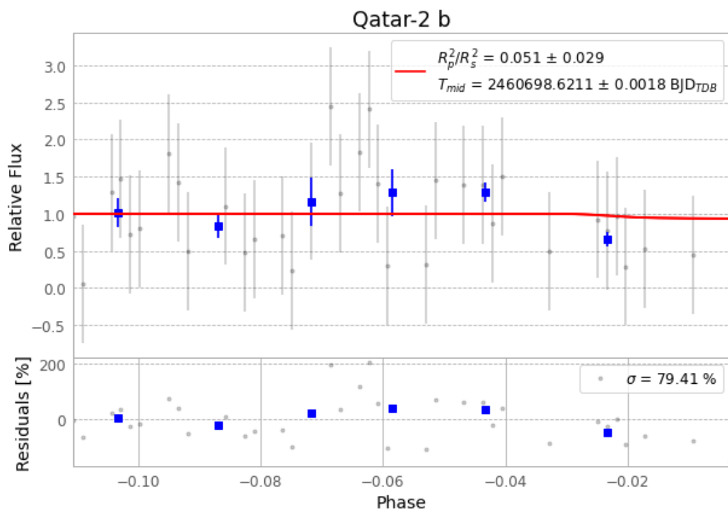
Figure 1 — FinalLightCurve_Qatar-2 b_2025-01-24.png (SHA-256 d09eb81b57d65df0...)
