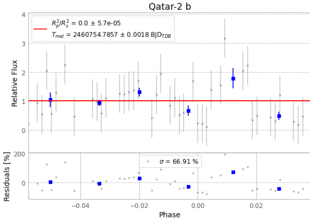
Figure 1 — FinalLightCurve_Qatar-2 b_2025-03-19.png (SHA-256 8a6968a71eaf4011...)
