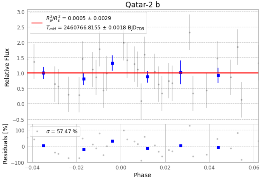
Figure 1 — FinalLightCurve_Qatar-2 b_2025-03-31.png (SHA-256 06f25ad621e22626...)
