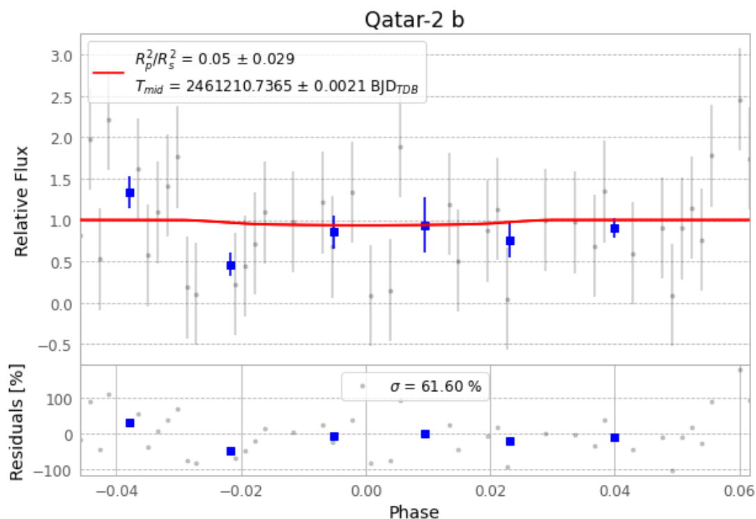
Figure 1 — FinalLightCurve_Qatar-2 b_2026-06-18.png (SHA-256 5a544b3d815ff6fe...)
