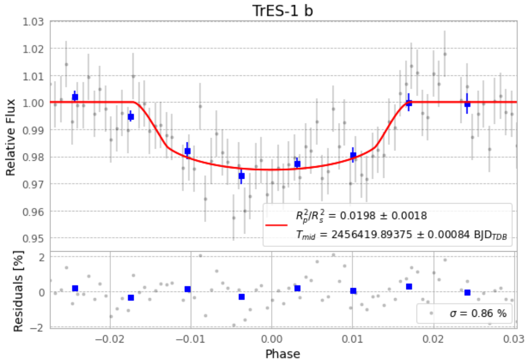
Figure 1 — FinalLightCurve_TrES-1 b_2013-05-07.png (SHA-256 abb034e8efd3e730...)
