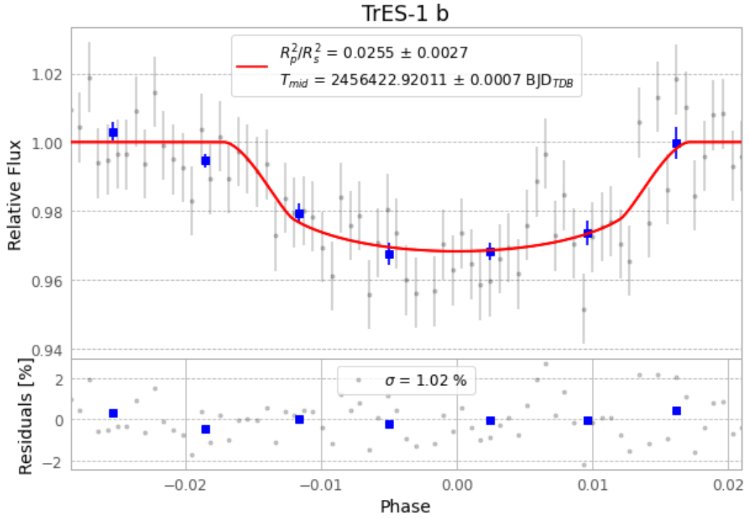
Figure 1 — FinalLightCurve_TrES-1 b_2013-05-10.png (SHA-256 e88787d147c931d3...)
