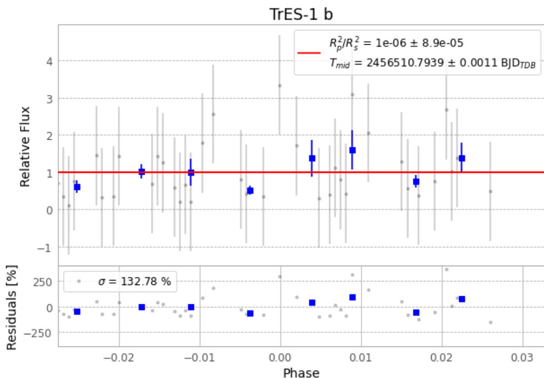
Figure 1 — FinalLightCurve_TrES-1 b_2013-08-05.png (SHA-256 fe92467b7909a90f...)
