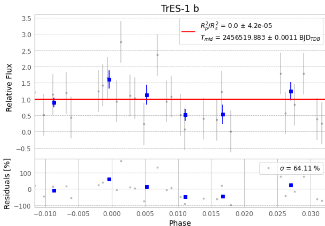
Figure 1 — FinalLightCurve_TrES-1 b_2013-08-15.png (SHA-256 7bde5eebe65e02d7...)
