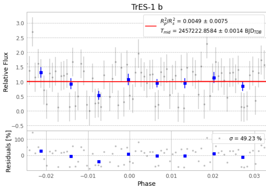
Figure 1 — FinalLightCurve_TrES-1 b_2015-07-18.png (SHA-256 99fa1e8daf0cf5db...)
