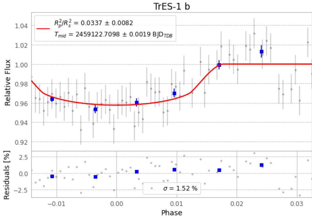
Figure 1 — FinalLightCurve_TrES-1 b_2020-09-29.png (SHA-256 ce2b17015cdd77c0...)
