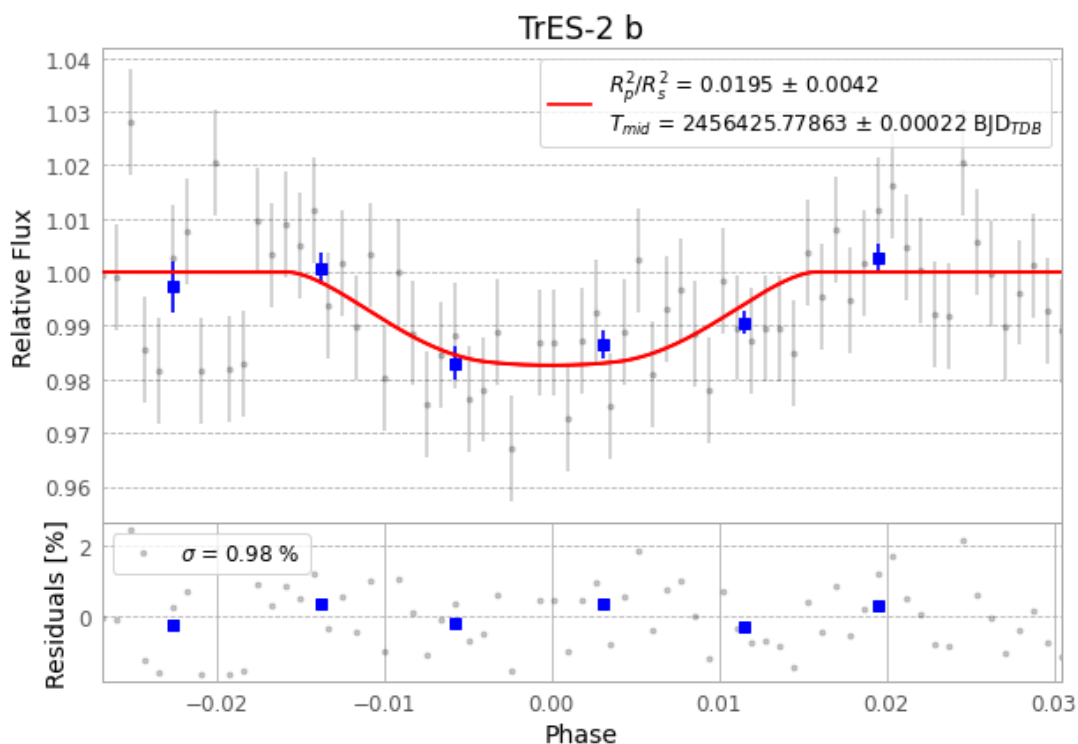
Figure 1 — FinalLightCurve_TrES-2 b_2013-05-12.png (SHA-256 49466c4be34eebbd...)
