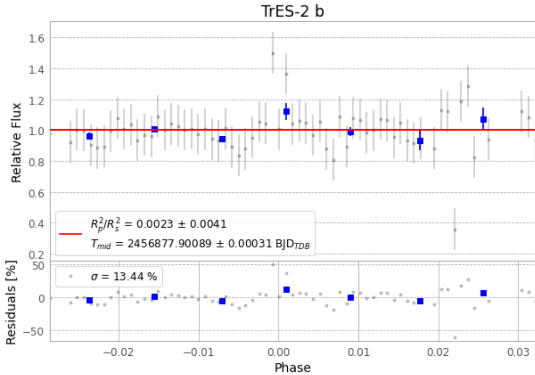
Figure 1 — FinalLightCurve_TrES-2 b_2014-08-08.png (SHA-256 0c244c777b034974...)
