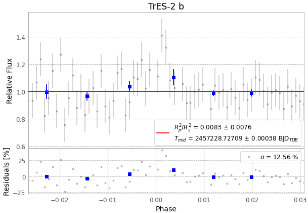
Figure 1 — FinalLightCurve_TrES-2 b_2015-07-24.png (SHA-256 80331a450dc53a6c...)
