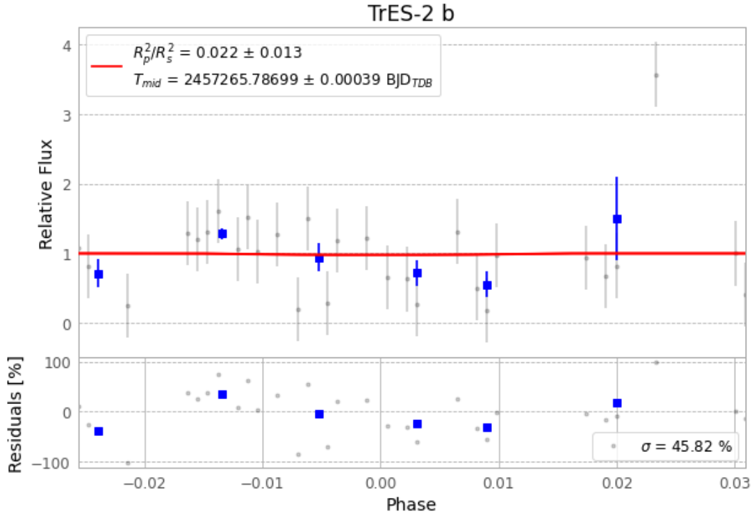
Figure 1 — FinalLightCurve_TrES-2 b_2015-08-30.png (SHA-256 457366313b0d08b4...)
