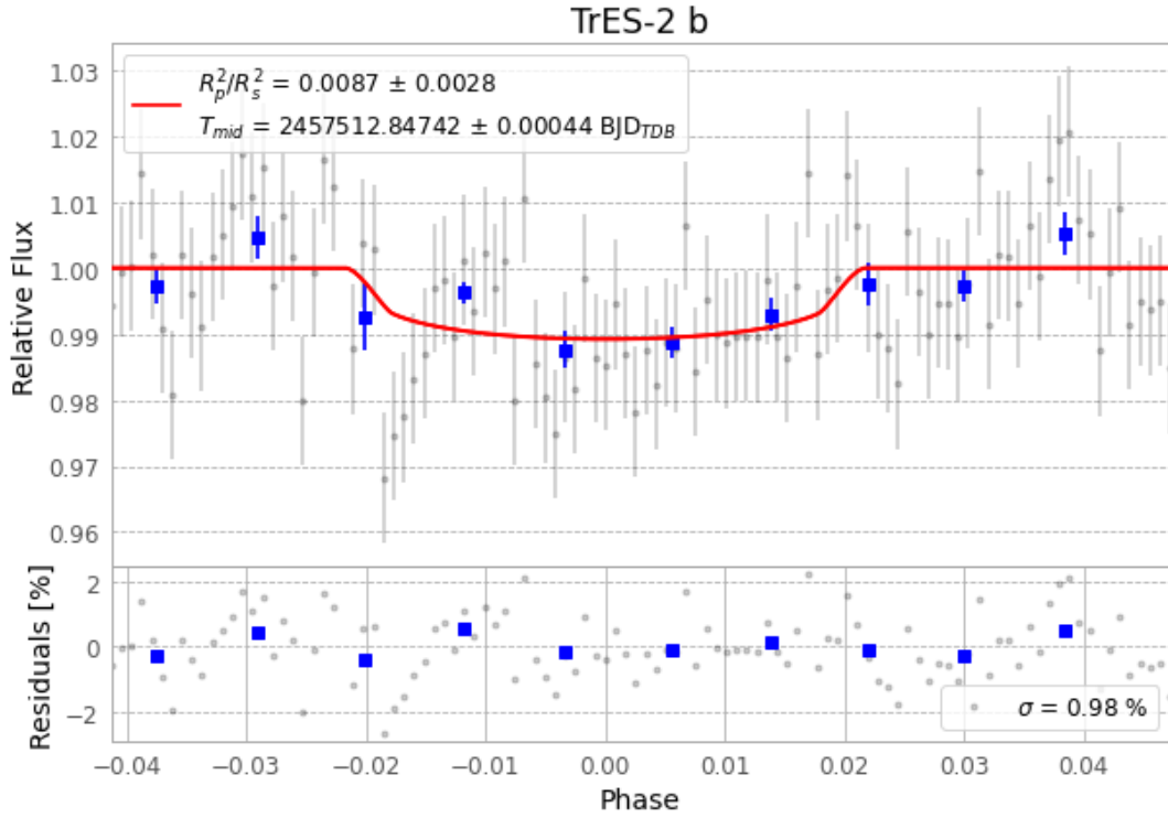
Figure 1 — FinalLightCurve_TrES-2 b_2016-05-03.png (SHA-256 a0cc43ebca69a8b7...)
