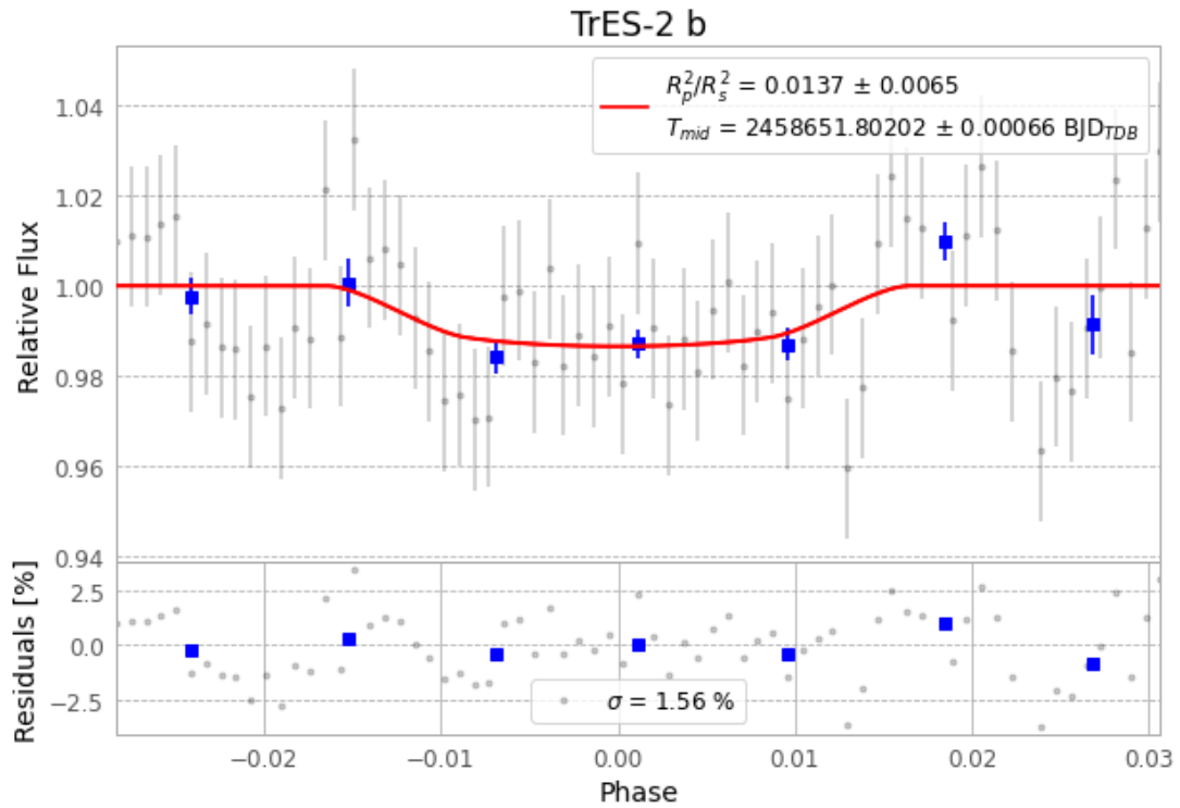
Figure 1 — FinalLightCurve_TrES-2 b_2019-06-16.png (SHA-256 662c0458503d1997...)
