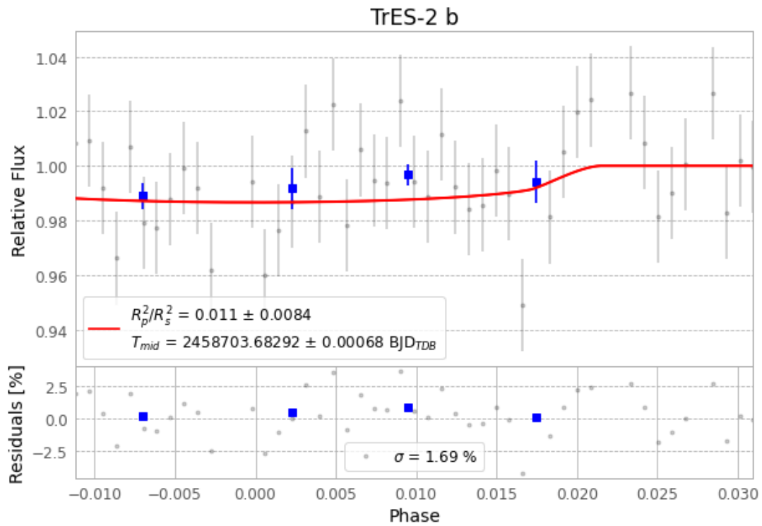
Figure 1 — FinalLightCurve_TrES-2 b_2019-08-07.png (SHA-256 27bf23d031053477...)
