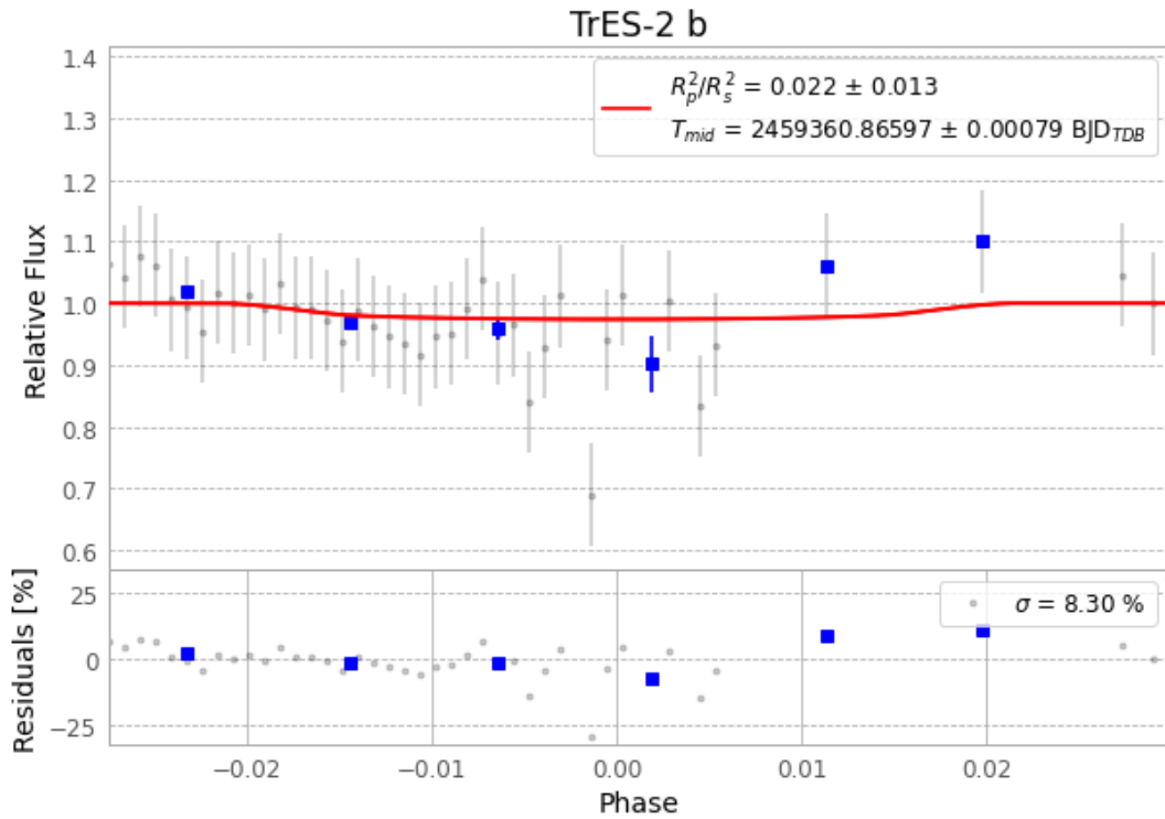
Figure 1 — FinalLightCurve_TrES-2 b_2021-05-26.png (SHA-256 469890adf3ab6d4c...)
