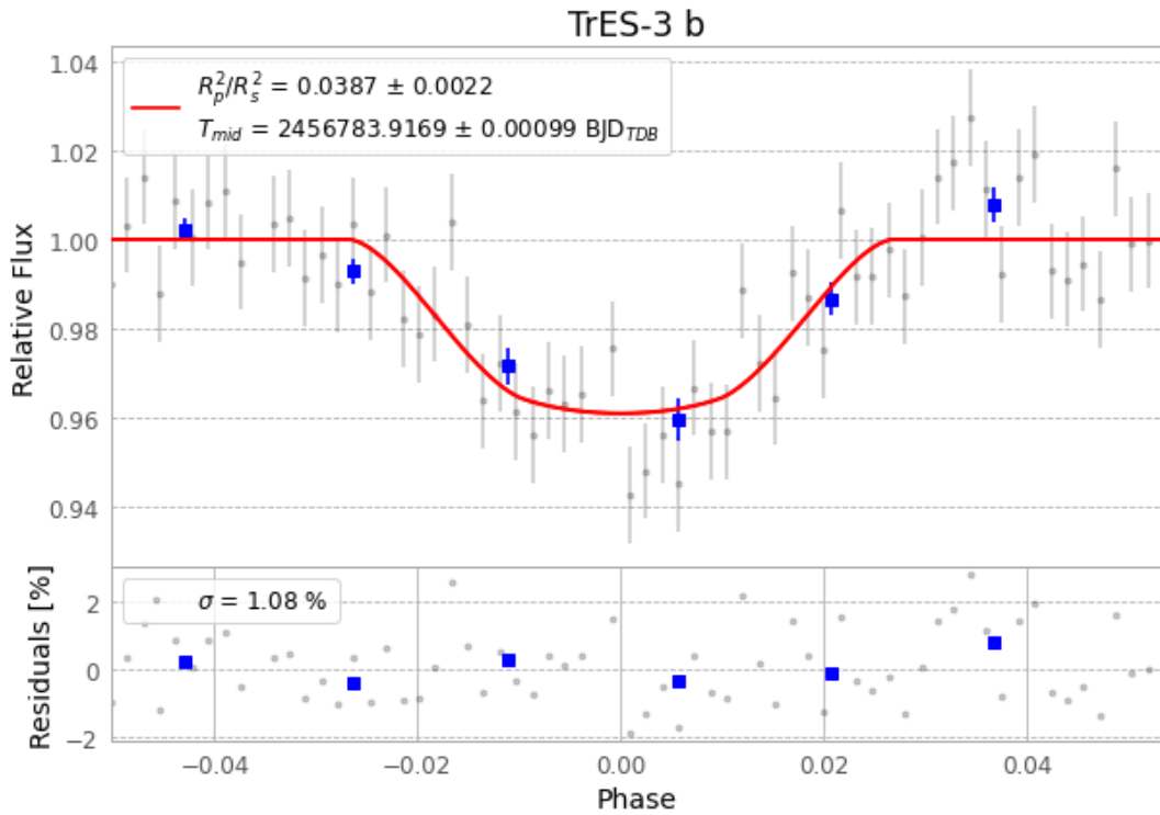
Figure 1 — FinalLightCurve_TrES-3 b_2014-05-06.png (SHA-256 1350877a2609224d...)
