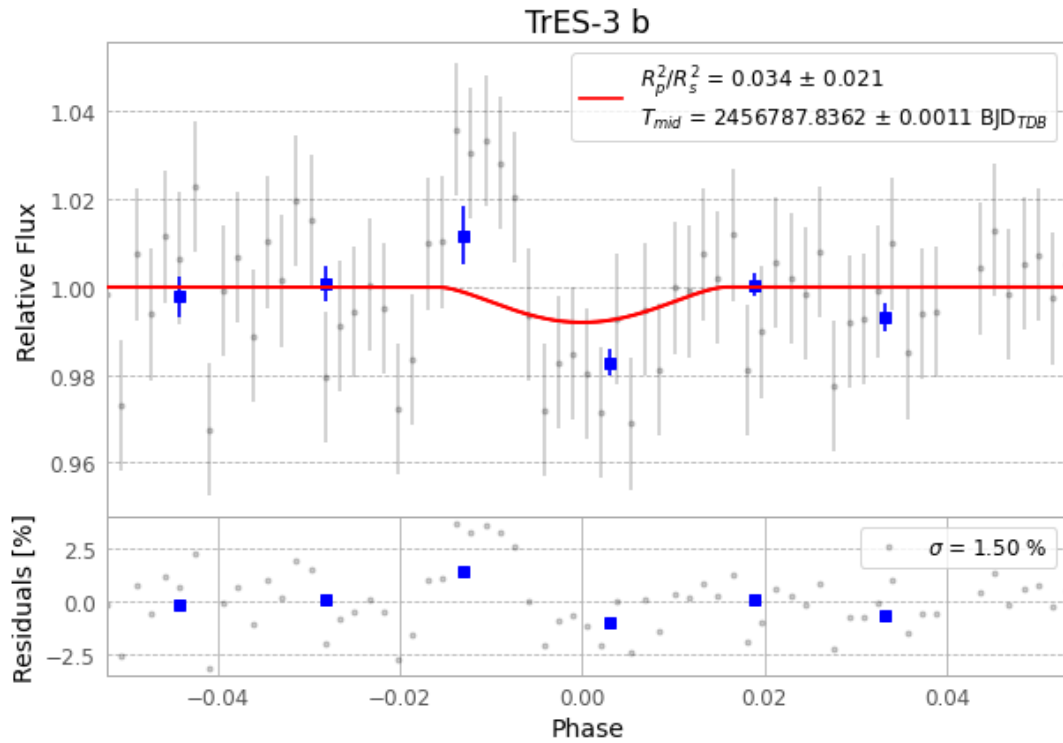
Figure 1 — FinalLightCurve_TrES-3 b_2014-05-09.png (SHA-256 11547e5067cbe48a...)
