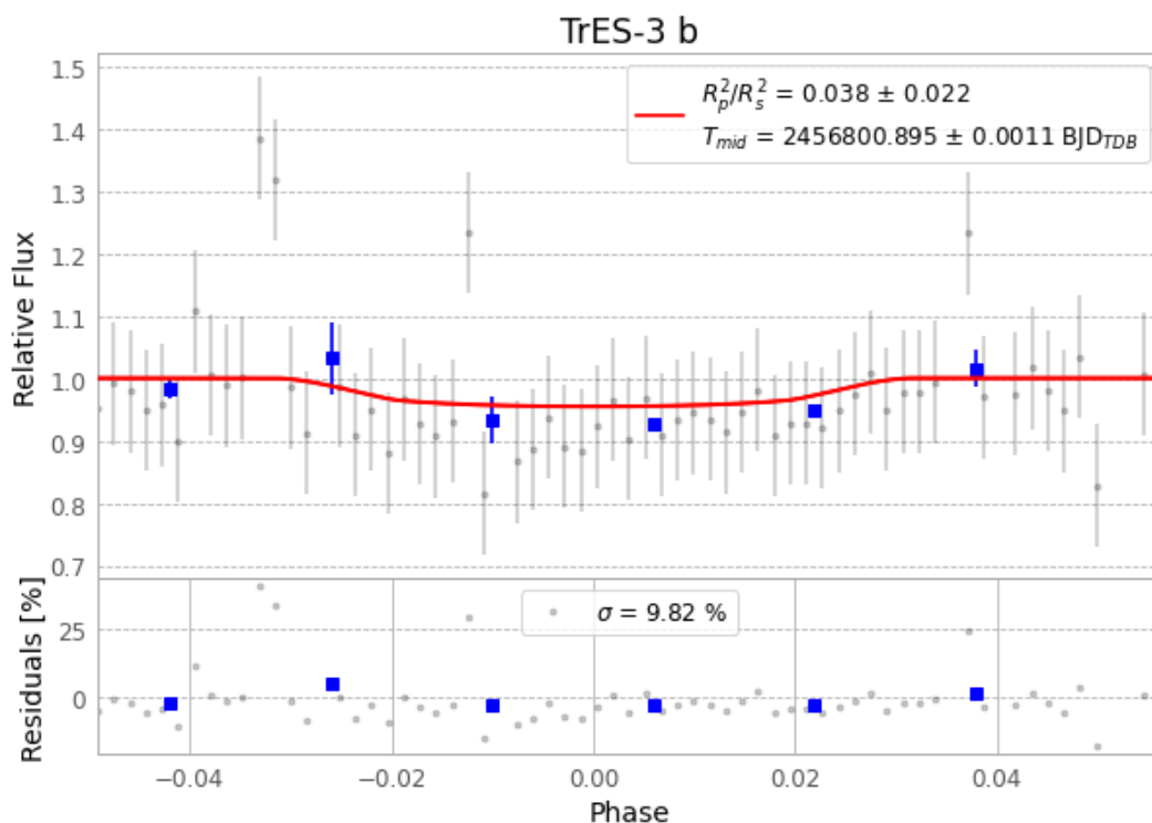
Figure 1 — FinalLightCurve_TrES-3 b_2014-05-23.png (SHA-256 0a0796248a53d367...)
