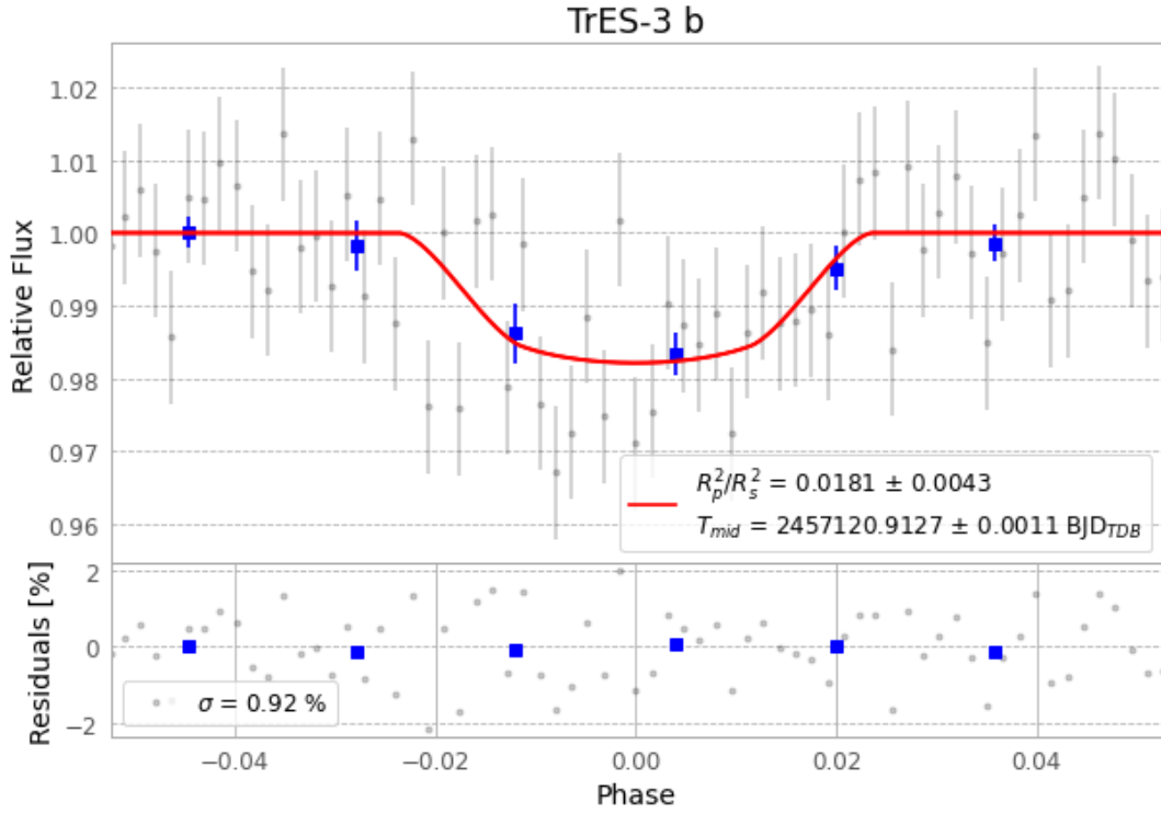
Figure 1 — FinalLightCurve_TrES-3 b_2015-04-08.png (SHA-256 aae90eb23048c749...)
