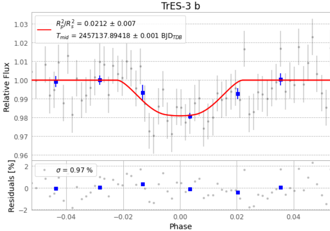
Figure 1 — FinalLightCurve_TrES-3 b_2015-04-25.png (SHA-256 35174f93922efbae...)
