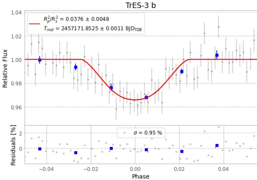
Figure 1 — FinalLightCurve_TrES-3 b_2015-05-28.png (SHA-256 9cb62289c301f0b9...)
