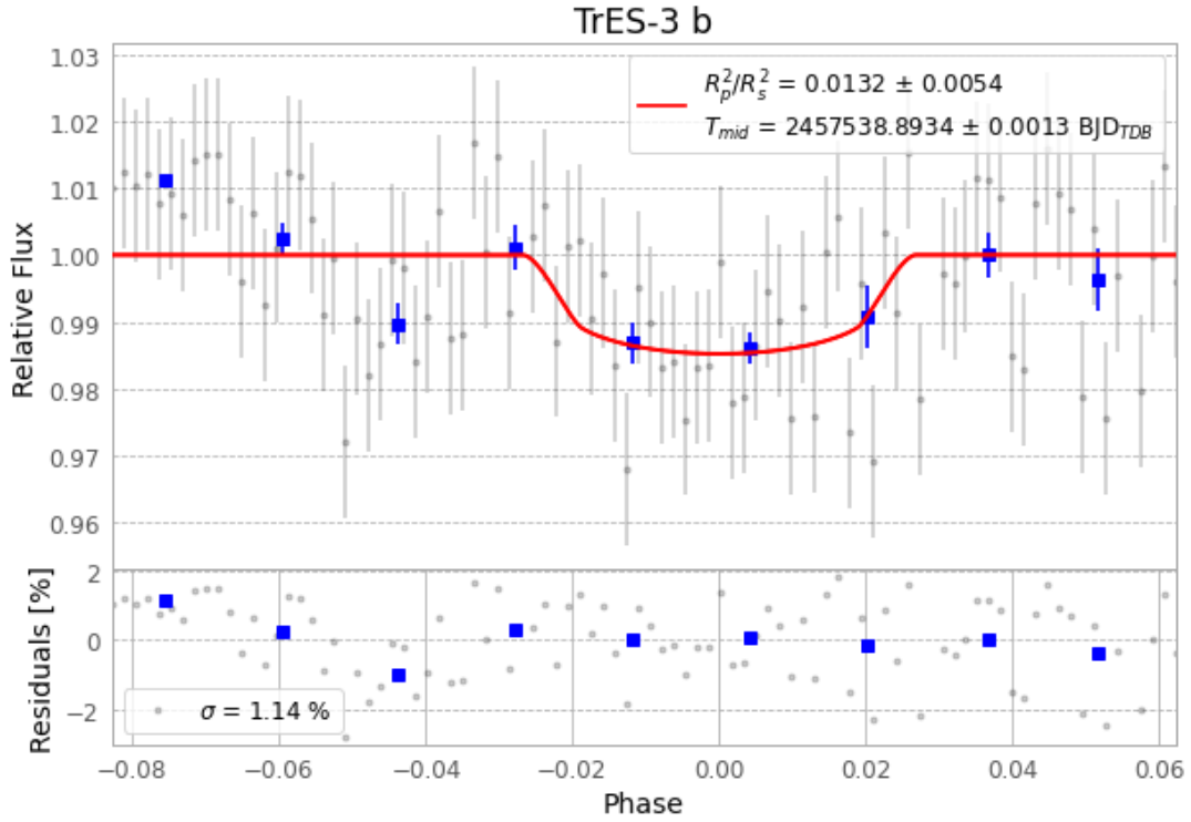
Figure 1 — FinalLightCurve_TrES-3 b_2016-05-29.png (SHA-256 69cc3b4b1568f4ba...)
