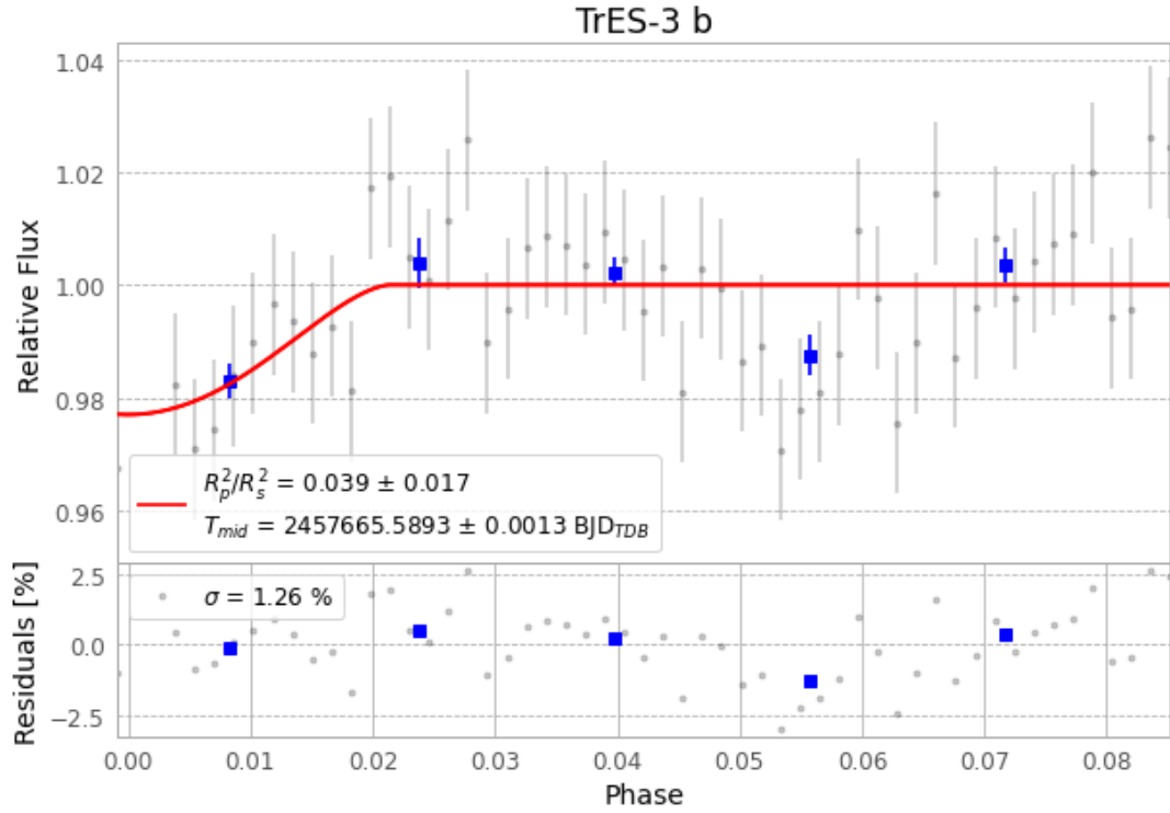
Figure 1 — FinalLightCurve_TrES-3 b_2016-10-03.png (SHA-256 579332b2dadca7f8...)
