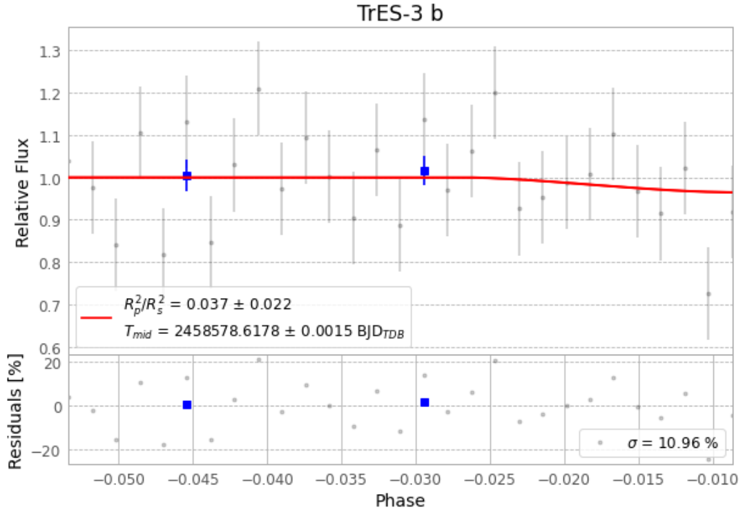
Figure 1 — FinalLightCurve_TrES-3 b_2019-04-06.png (SHA-256 d8f46af190290449...)
