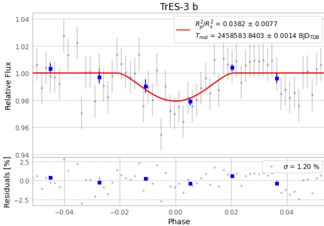
Figure 1 — FinalLightCurve_TrES-3 b_2019-04-09.png (SHA-256 84762d8cc15fe541...)
