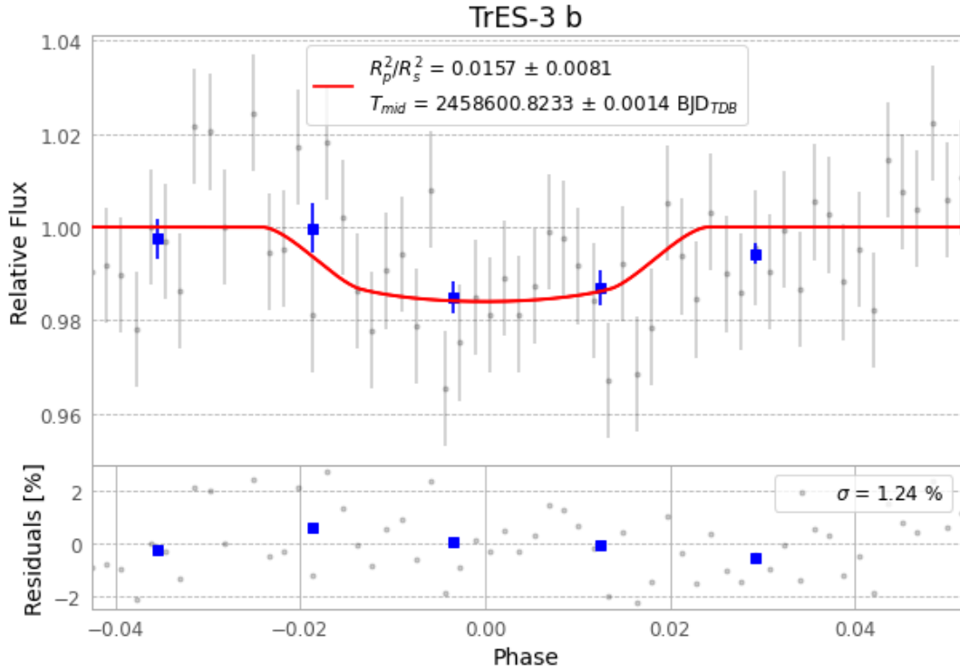
Figure 1 — FinalLightCurve_TrES-3 b_2019-04-26.png (SHA-256 4061c41a8e866b54...)
