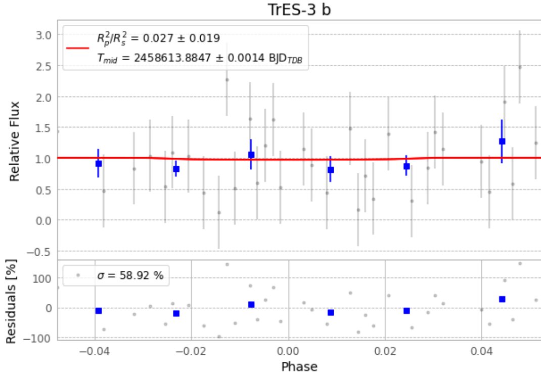
Figure 1 — FinalLightCurve_TrES-3 b_2019-05-10.png (SHA-256 f0f76416b5cfef9a...)
