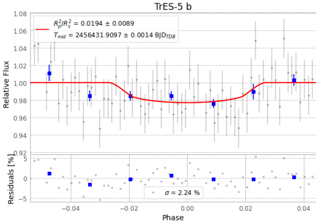
Figure 1 — FinalLightCurve_TrES-5 b_2013-05-19.png (SHA-256 d378a9fe8b0ba595...)
