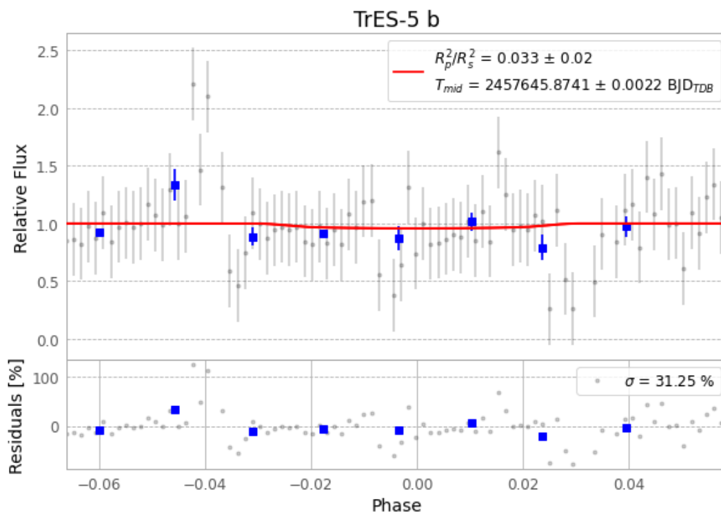
Figure 1 — FinalLightCurve_TrES-5 b_2016-09-13.png (SHA-256 434c35bbeafd4667...)
