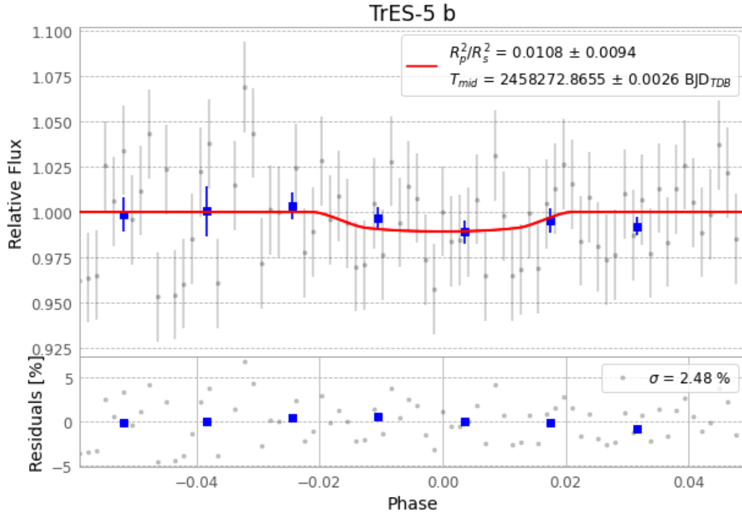
Figure 1 — FinalLightCurve_TrES-5 b_2018-06-02.png (SHA-256 0ebd76fa84c887d3...)
