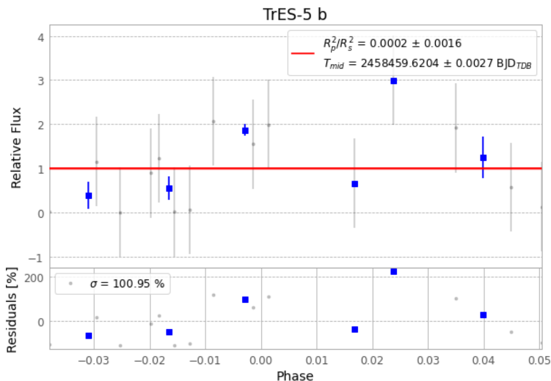
Figure 1 — FinalLightCurve_TrES-5 b_2018-12-06.png (SHA-256 255b328c48884045...)
