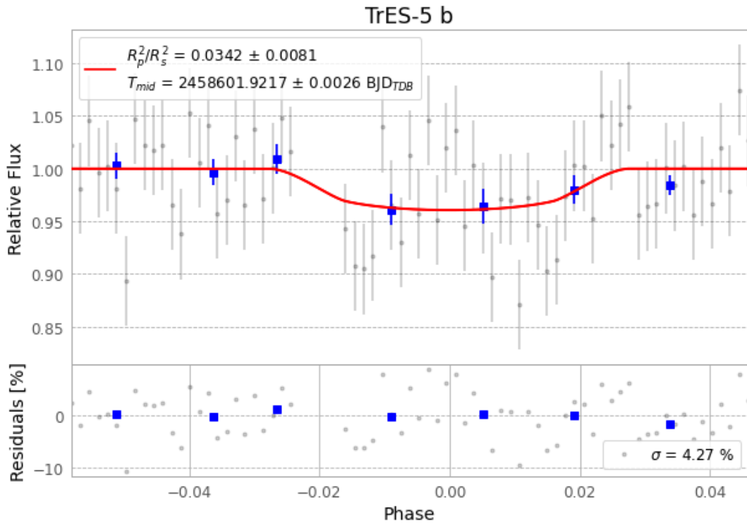
Figure 1 — FinalLightCurve_TrES-5 b_2019-04-28.png (SHA-256 3b3d6366ec2799fd...)
