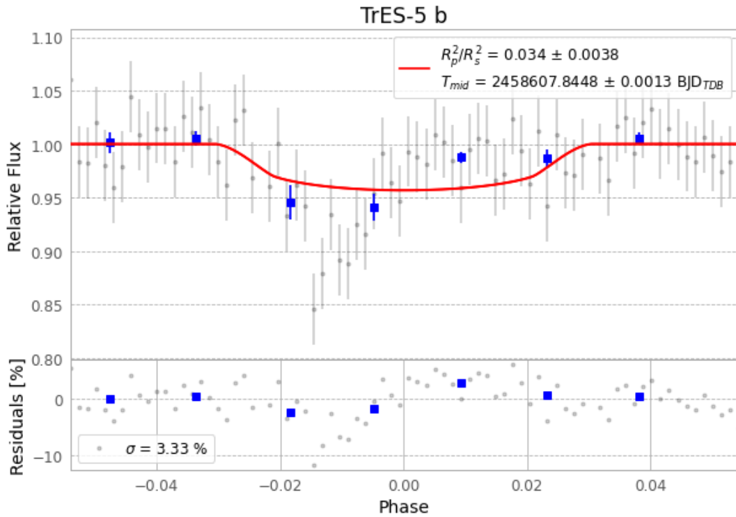
Figure 1 — FinalLightCurve_TrES-5 b_2019-05-03.png (SHA-256 242fecdd98bd4166...)
