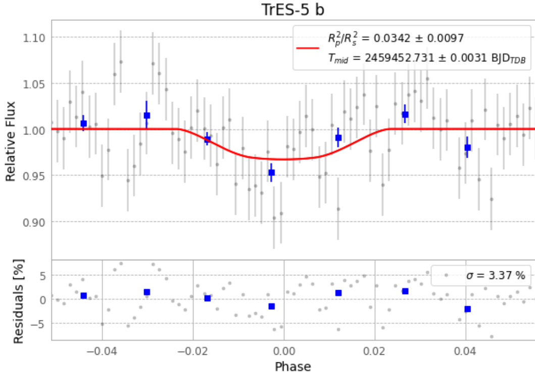
Figure 1 — FinalLightCurve_TrES-5 b_2021-08-25.png (SHA-256 842f8b76578c17aa...)
