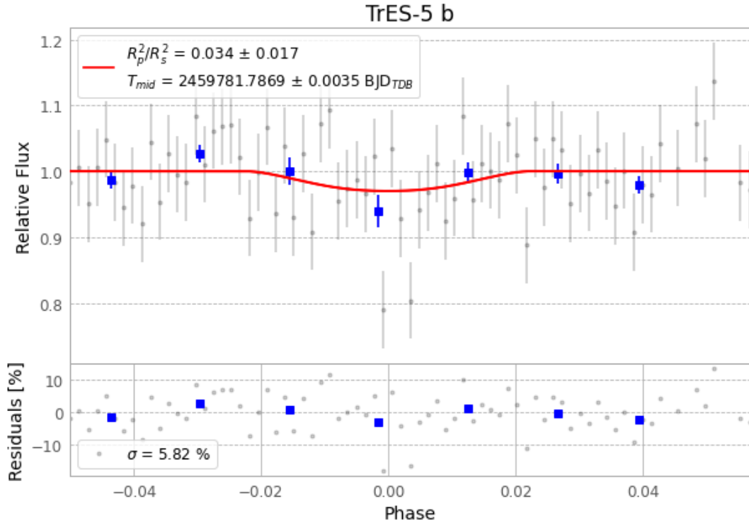
Figure 1 — FinalLightCurve_TrES-5 b_2022-07-20.png (SHA-256 4e711a35a3af7e6e...)
