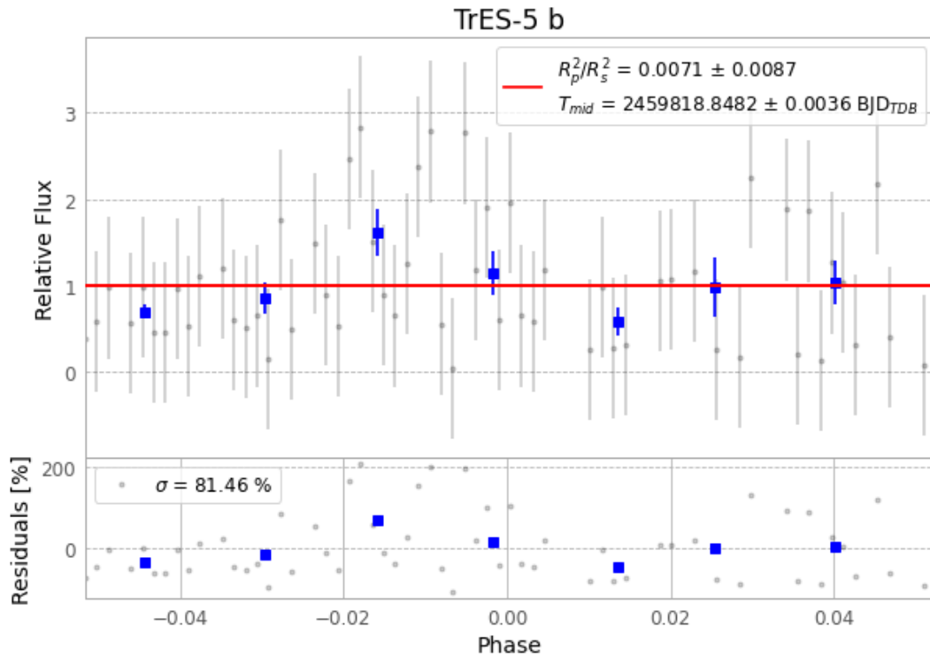
Figure 1 — FinalLightCurve_TrES-5 b_2022-08-26.png (SHA-256 c6a00bd4131a6439...)
