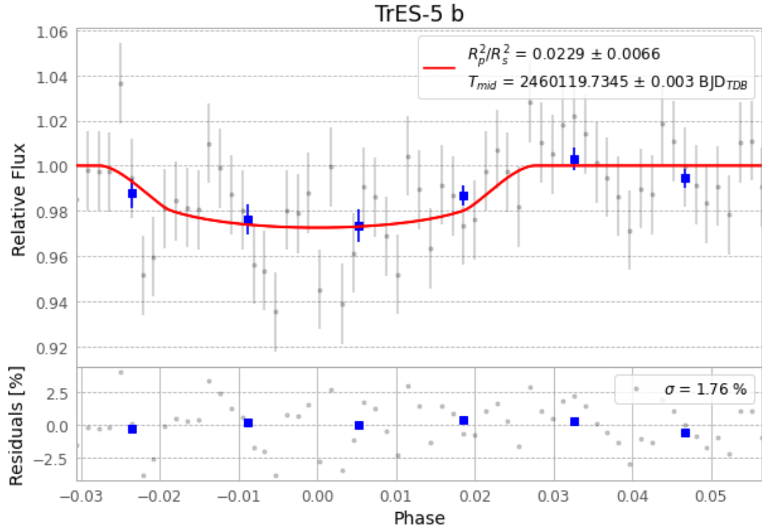
Figure 1 — FinalLightCurve_TrES-5 b_2023-06-23.png (SHA-256 28aa3efbea0216ea...)
