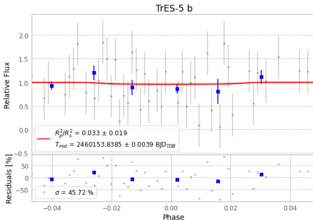
Figure 1 — FinalLightCurve_TrES-5 b_2023-07-27.png (SHA-256 c3069217cc5e5010...)
