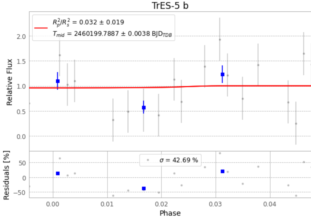
Figure 1 — FinalLightCurve_TrES-5 b_2023-09-11.png (SHA-256 a6296c45c2394c4a...)
