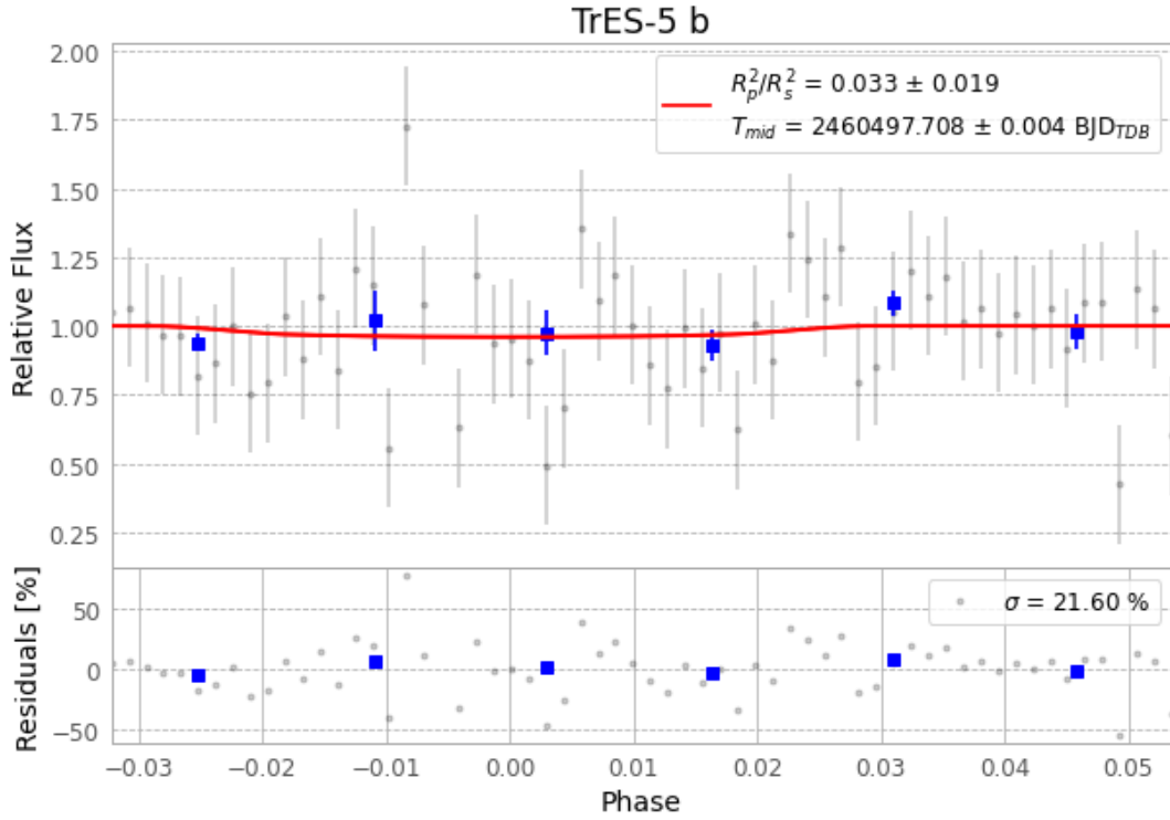
Figure 1 — FinalLightCurve_TrES-5 b_2024-07-05.png (SHA-256 3e25a3e025ac89d7...)
